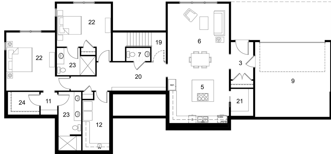
LOWER LEVEL FLOOR PLAN 1/16" = 1'
